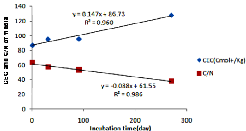
Figure 1. Changes of CEC and C/N ratio of palm media under incubation time.
